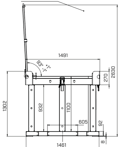
ASP 1 800 11AX
