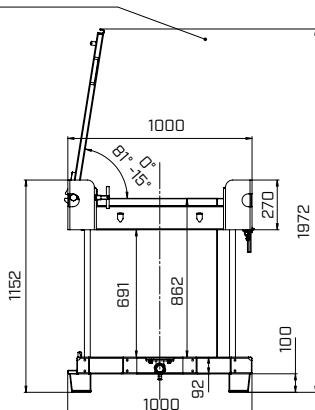
ASP 600 11AX
